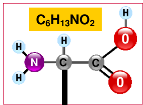
Side Chain R
