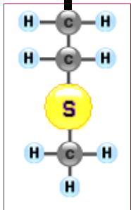
Side Chain R
