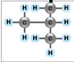
Side Chain R
