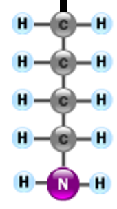
Side Chain R
